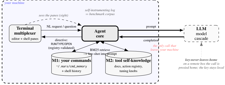
Figure 1: MARS retrieves with lexical BM25 from two local stores (M1, the user’s past commands; M2, the tool’s own docs and registry) and injects the results as few-shot exemplars. Only the model call leaves the machine; on a remote box even the key stays home, and every call is logged.
