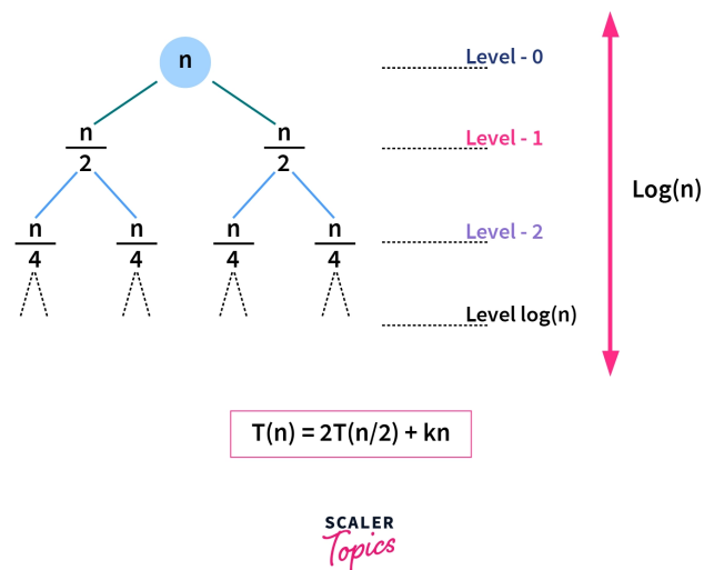
Figure 6.1: Recursion Tree
