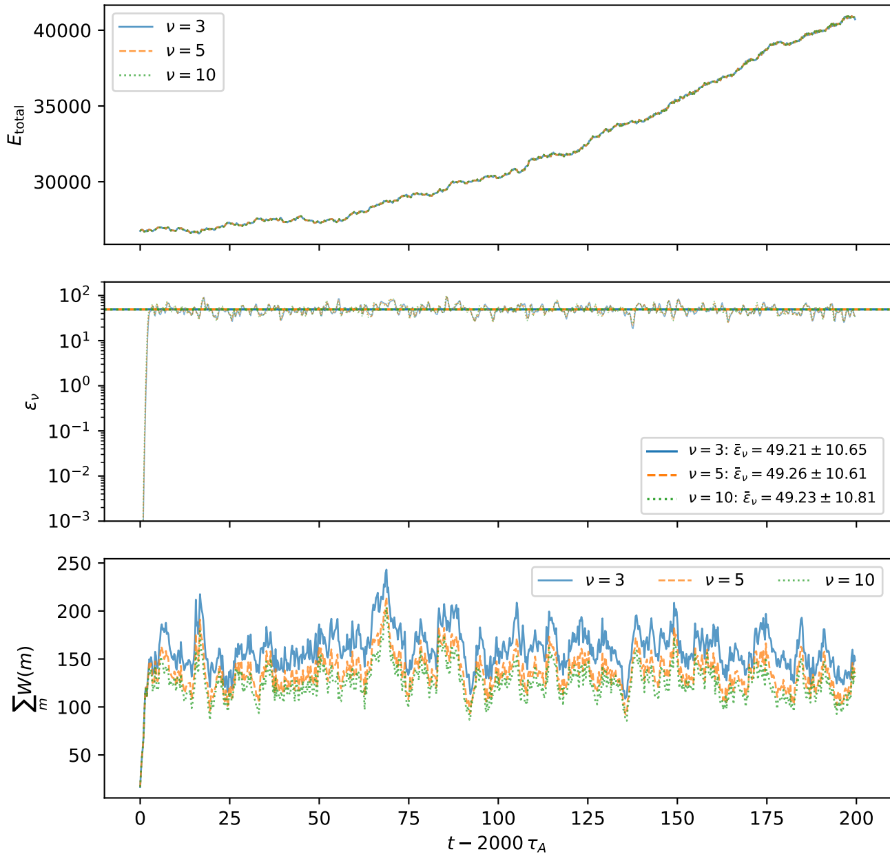
IMEX-RK222 \nu -scan at M = 128 , 200 \tau_A from Alfvénic t = 2000
