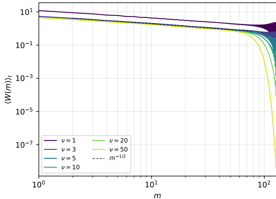
Hermite spectrum across the \nu -scan
