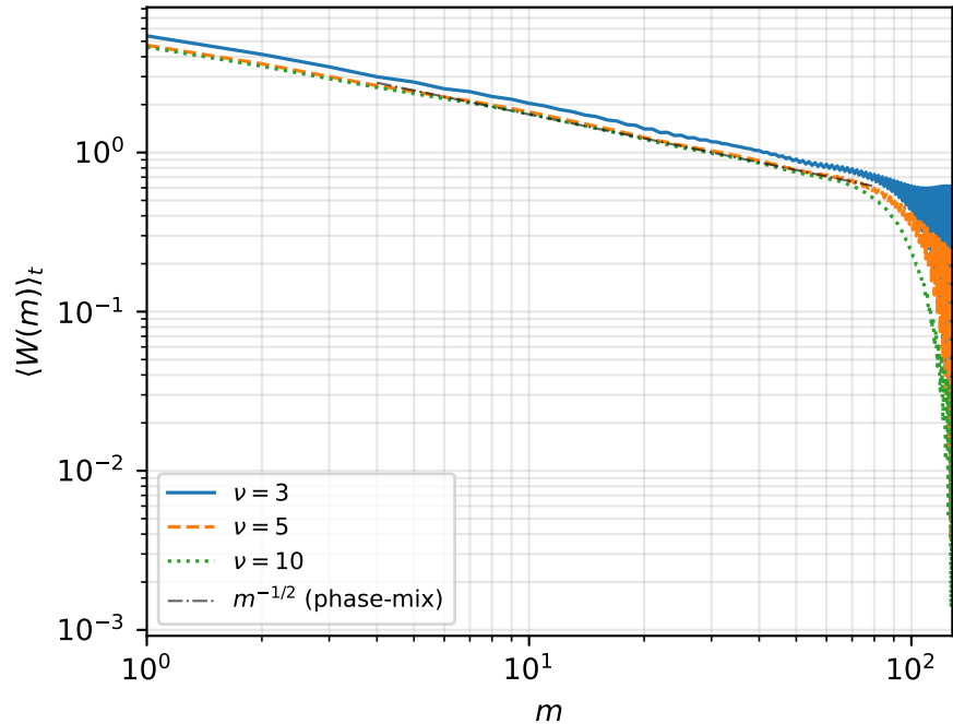
Time-averaged Hermite spectrum (t=2100--2200)
