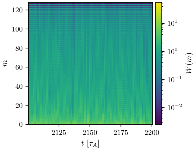
(b) Hermite spectrum W(m, t)
