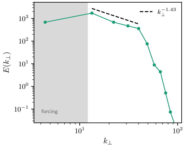
(a) base-state perpendicular spectrum
