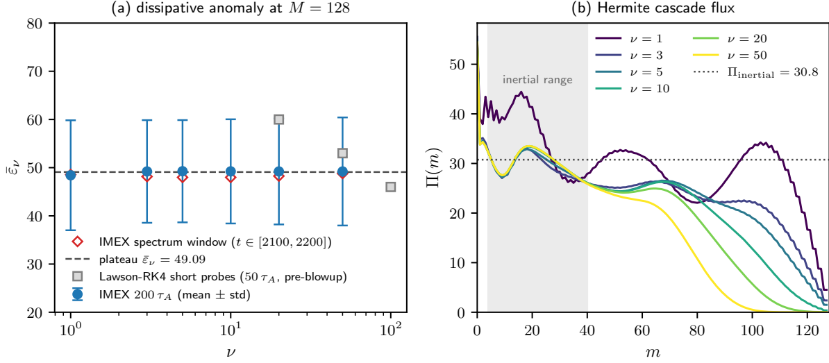
Figure 1: Dissipative anomaly and constant-flux cascade. Left: time-averaged collisional dissipation \bar{\varepsilon}_\nu as a function of \nu , from six IMEX runs at M = 128 , 128^3 , 200\tau_A . Blue circles are time-series means with \pm 1\sigma error bars; red diamonds are spectrum-window means. The horizontal dashed line at \bar{\varepsilon}_\nu = 49.09 is the six-point mean. Gray squares are legacy Lawson-RK4 short-probe points ( 50\tau_A before numerical blowup set in; see Appendix A) and are shown for reference only. Right: time-averaged Hermite cascade flux \Pi(m) = \sum_{\mathbf{k}} \Gamma_{m,\mathbf{k}} , where \Gamma_{m,\mathbf{k}} = -k_\parallel \sqrt{2(m+1)} \text{Im}[g_{m+1}g_m^*] , averaged over checkpoints at t = 2180, 2190, 2200\tau_A . Colours run from \nu = 1 (purple) to \nu = 50 (yellow). The inertial range m \in [4, 40] is shaded; in that range \Pi(m) is approximately constant in m and approximately the same across all six \nu , with a six-point mean \Pi_{\text{inertial}} = 30.8 . Beyond the inertial range the curves split with the dissipation-scale ordering: lower \nu carries the cascade further out in m before collisions absorb it.
