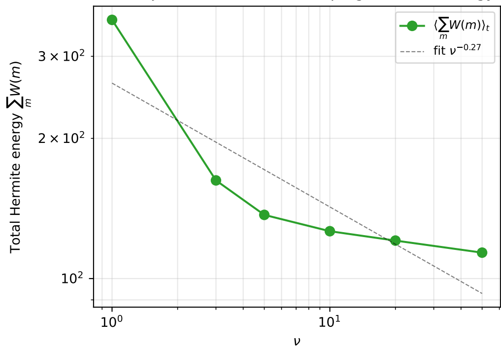
Self-adjustment: weaker damping \rightarrow more energy
