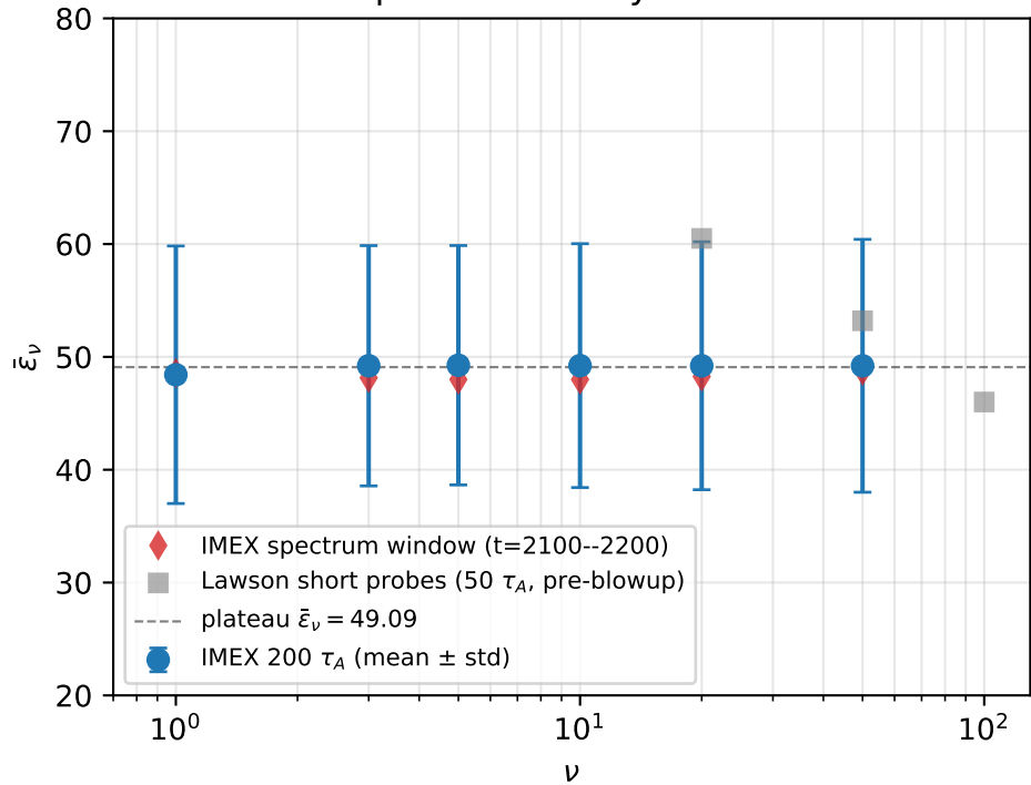
Dissipative anomaly at M = 128
