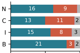
Qwen-Next / MiniSWE
