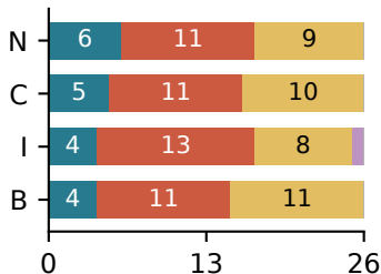
Qwen-Next / MiniSWE
