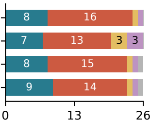
Qwen-30B / MiniSWE
