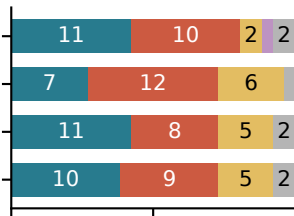
Qwen-30B / MiniSWE
