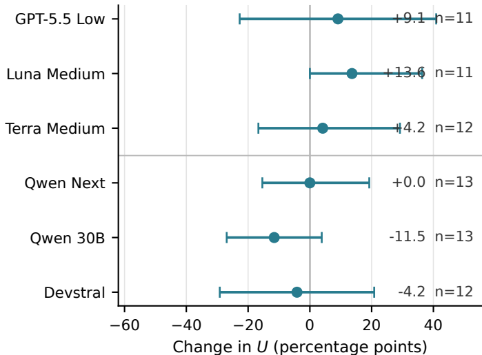
Correct memory vs. no memory (C–N)
