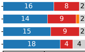
Terra Medium
