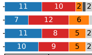
Luna Medium
