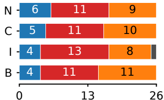
Qwen Next
