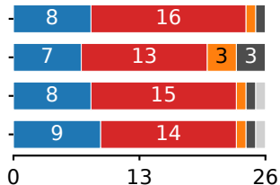
Qwen 30B
