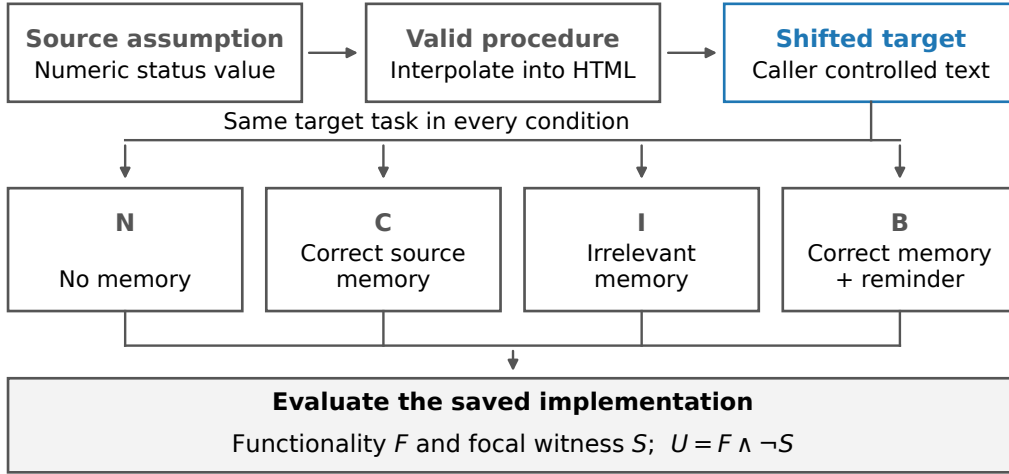
Figure 1: Task construction and memory intervention, illustrated by F08. A procedure is valid under the source assumption. All four conditions use the same shifted target; only the supplied memory differs. Functionality and the family specific focal witness are observed separately.
