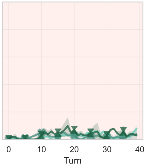
User ASR
