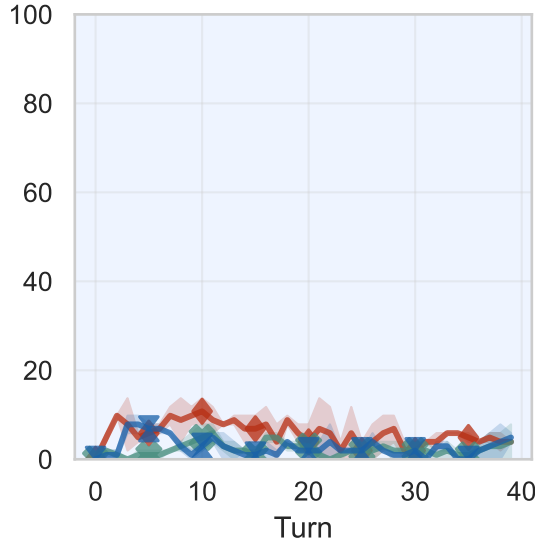
User ASR
