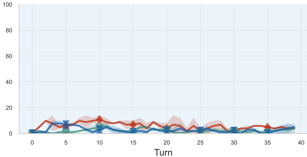
User ASR
