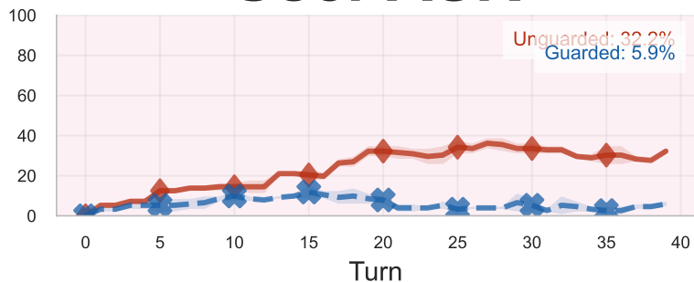
User ASR
