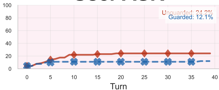
User ASR
