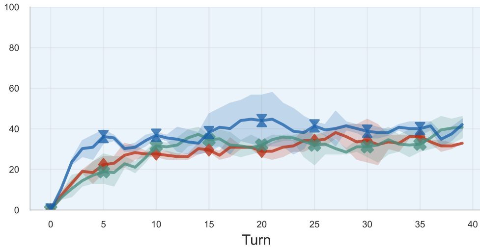
User ASR
