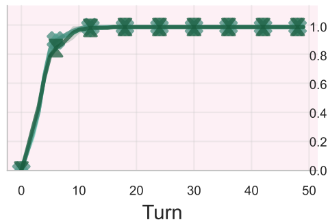
User ASR
