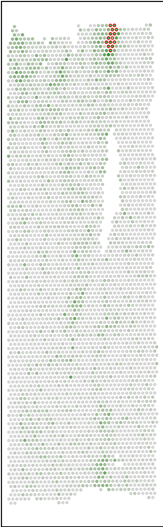
CD4_S02
