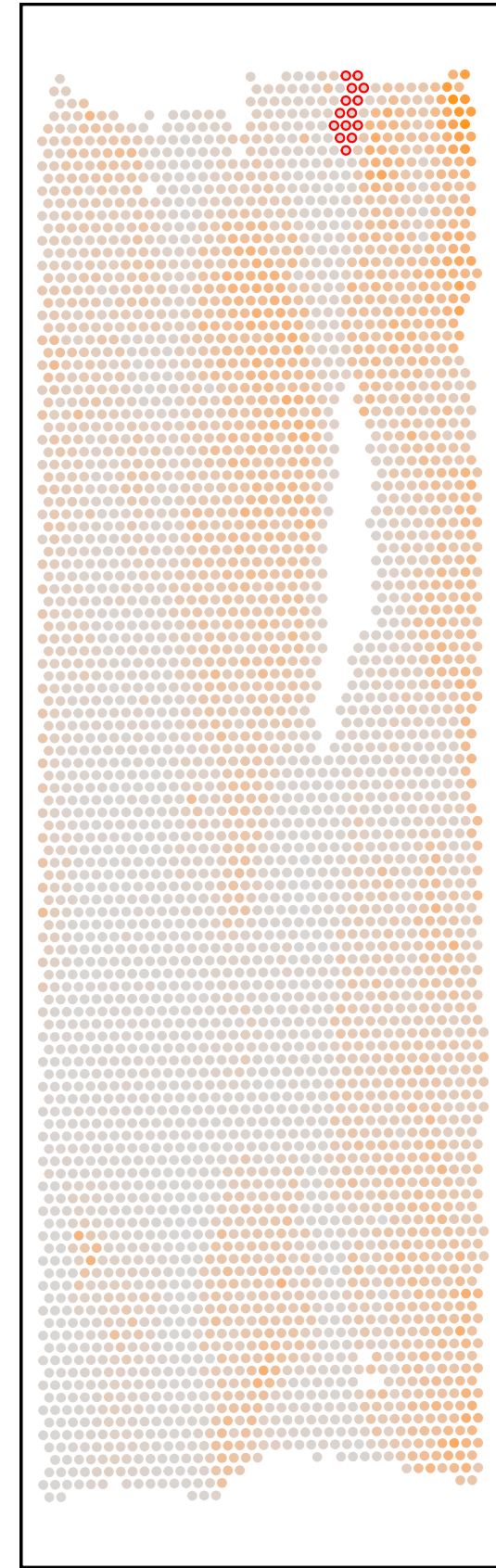
Cancer Cells
