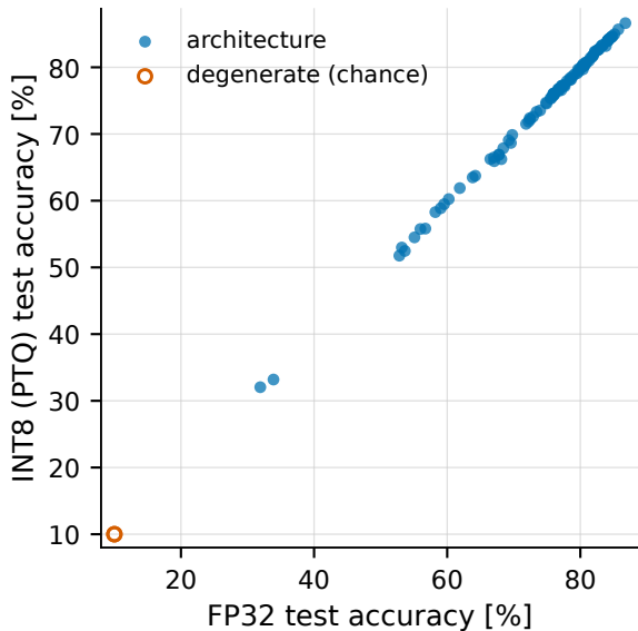
(a) Quantization preserves accuracy
