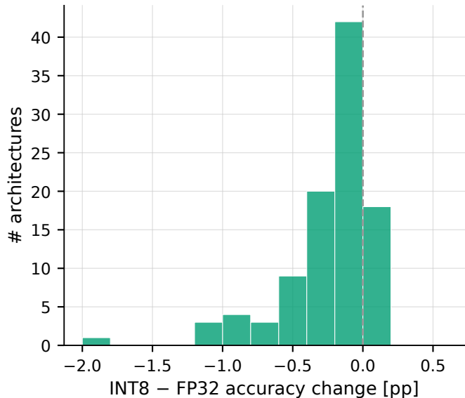
(b) Quantization barely moves accuracy
