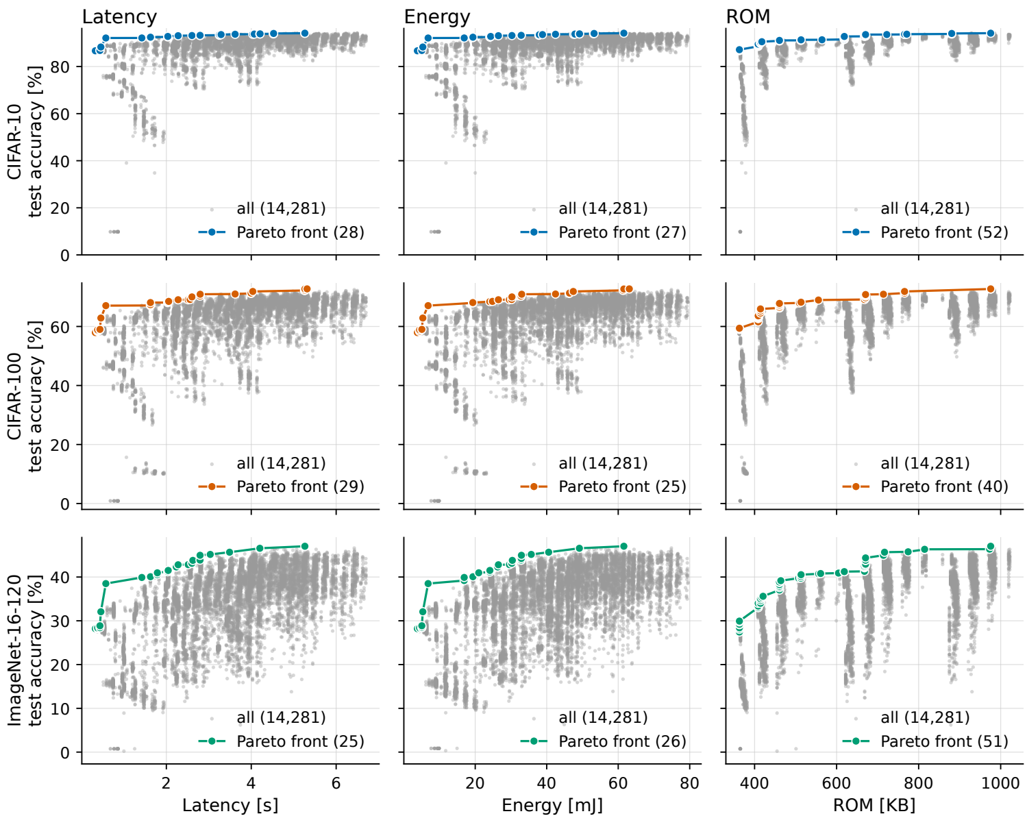
Accuracy vs. hardware cost — Pareto frontiers per dataset
