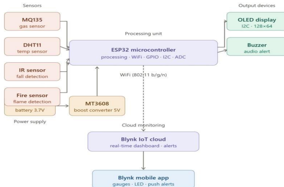
Figure 3.1 : Block Diagram of IoT Smart Helmet
