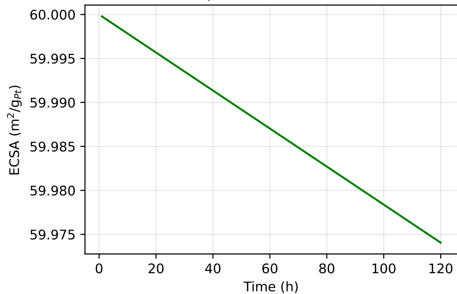
Catalyst Surface Area Loss
