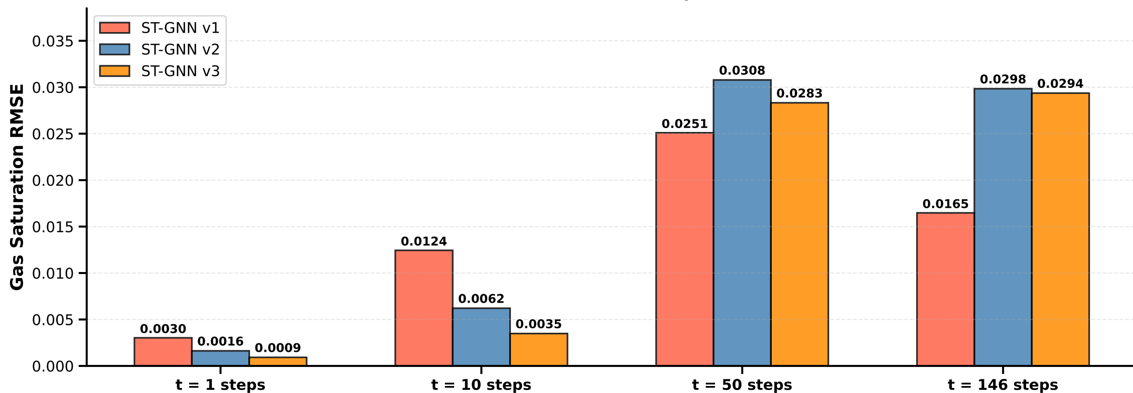
Gas Saturation Rollout Error ( S_g ) at Checkpoints
