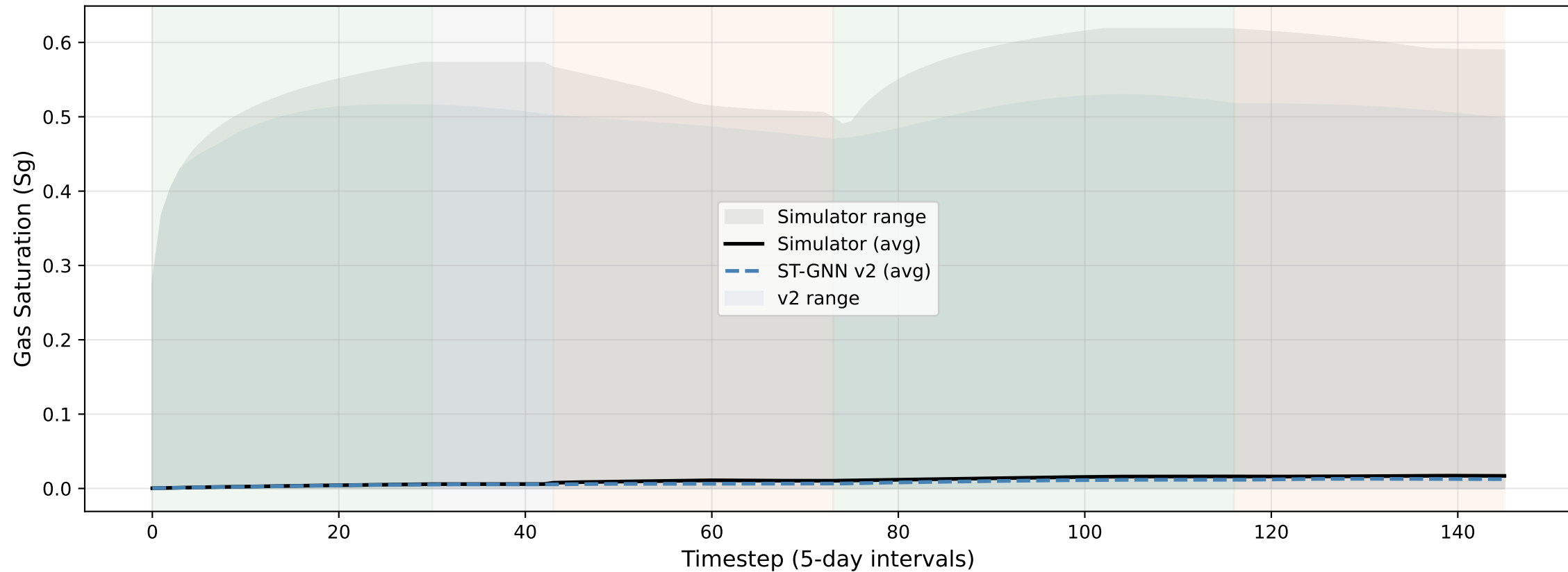
Gas Saturation Tracking: ST-GNN v2 vs Reservoir Simulator (Case 5, shading = field min/max range)
