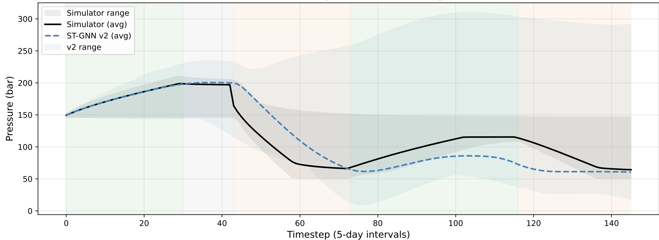
Pressure Field Tracking: ST-GNN v2 vs Reservoir Simulator (Case 5, shading = field min/max range)
