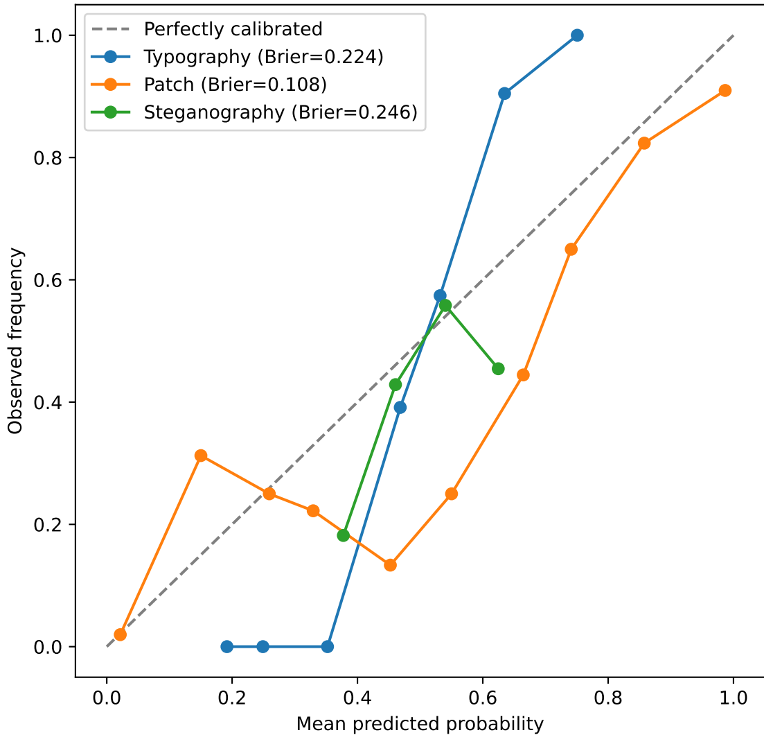
Reliability Diagram (all heads)
