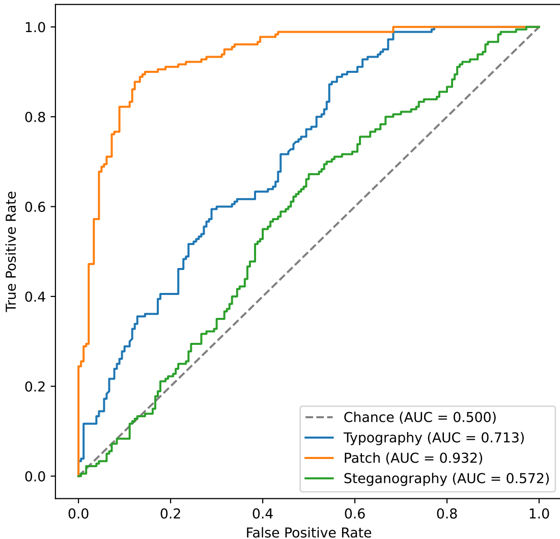
ROC Curves — All Heads
