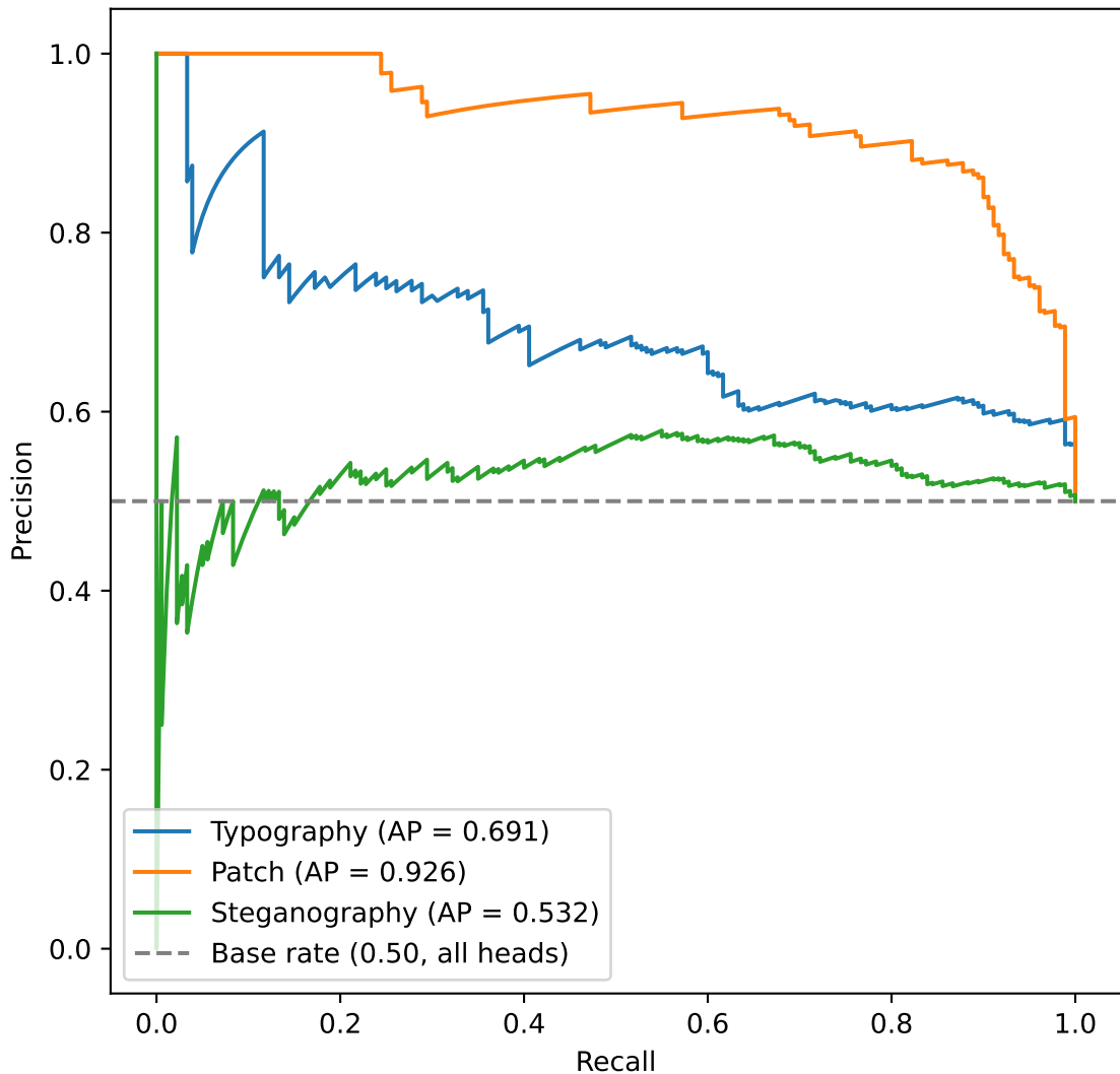
Precision-Recall Curves — All Heads
