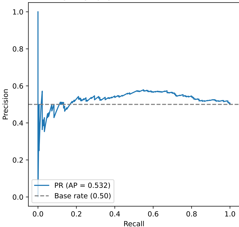
Steganography — Precision-Recall Curve
