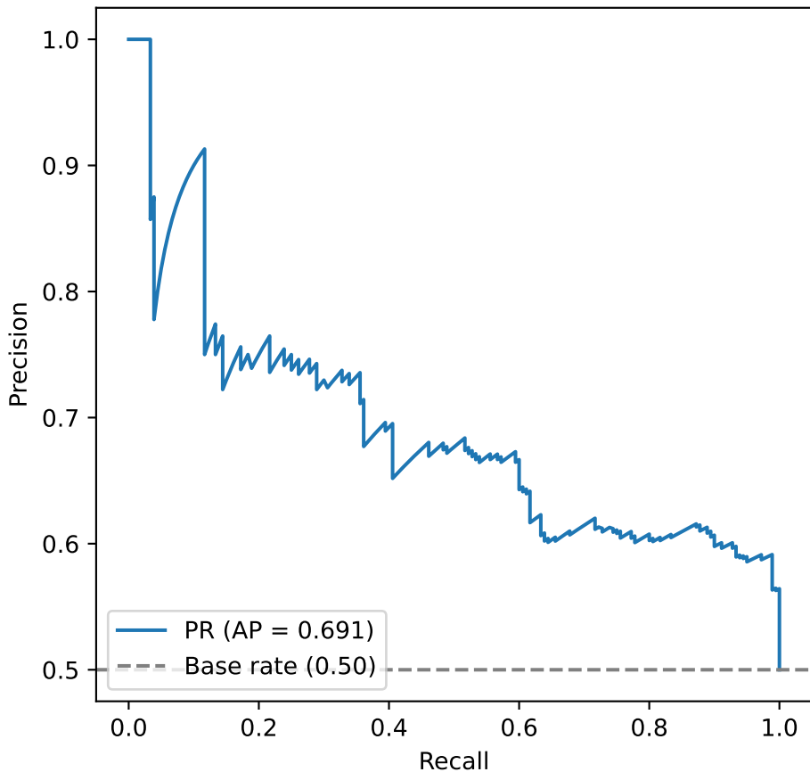
Typography — Precision-Recall Curve
