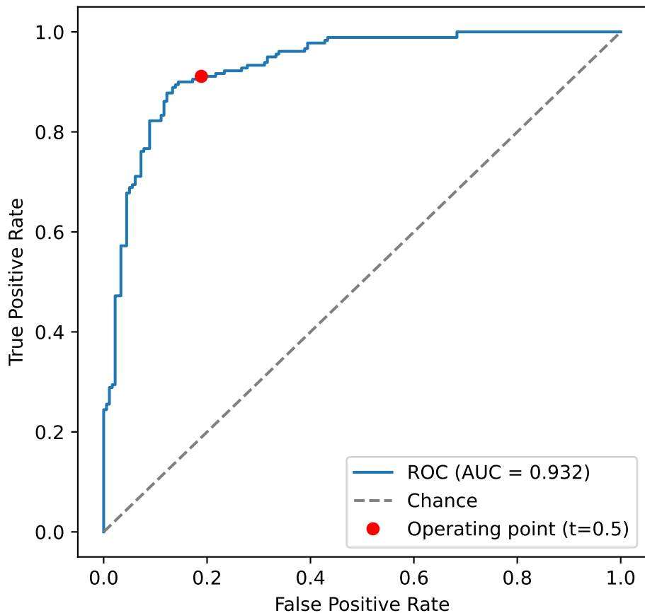
Patch — ROC Curve
