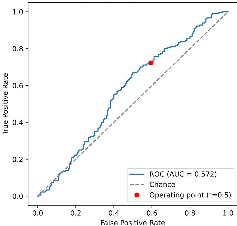
Steganography — ROC Curve
