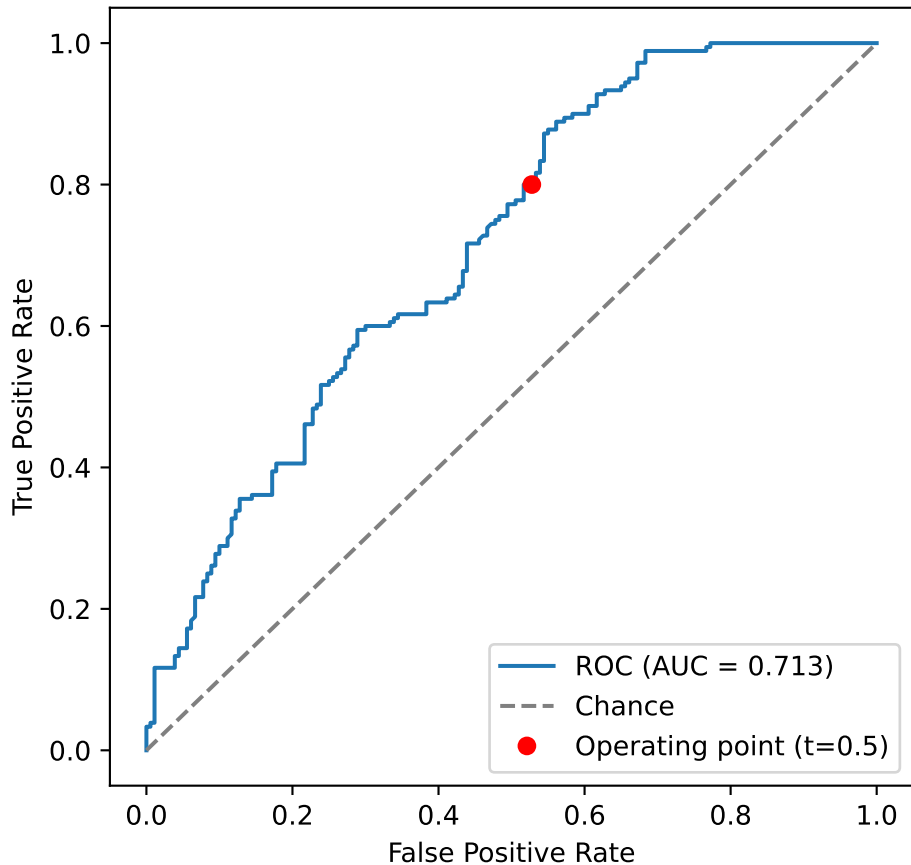
Typography — ROC Curve
