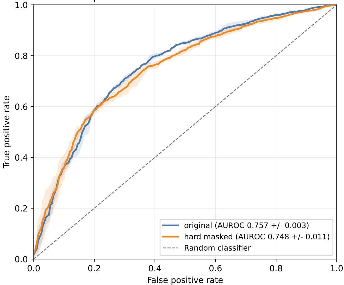
CheXpert validation: mean ROC across 3 seeds
