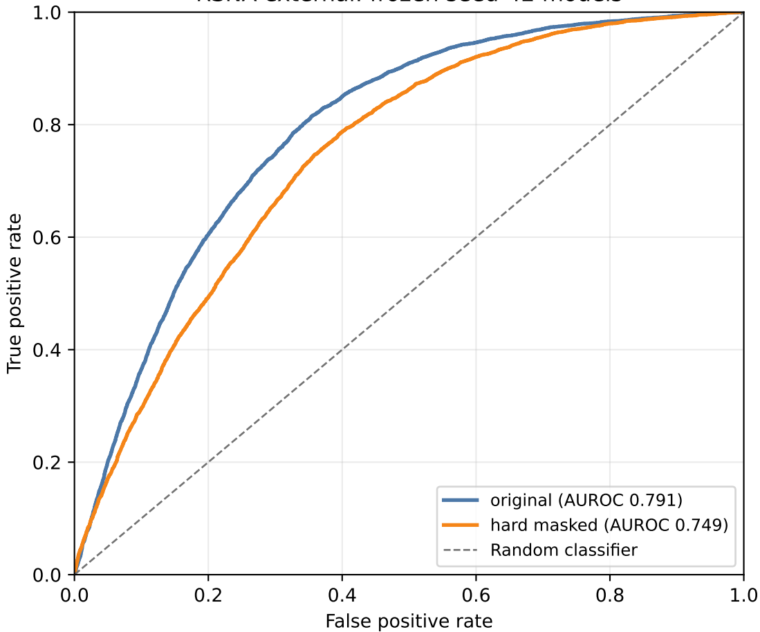
RSNA external: frozen seed-42 models
