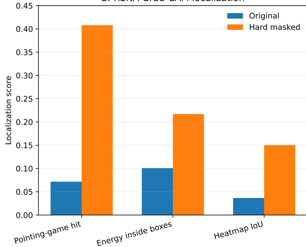
B. RSNA Grad-CAM localization
