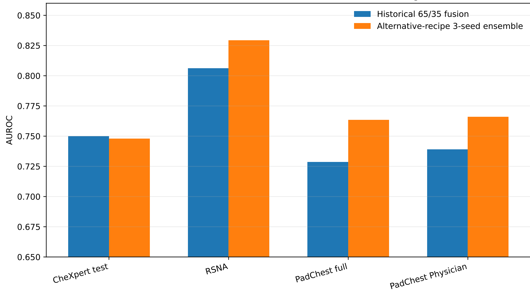
Cross-dataset discrimination of frozen ResNet50 strategies
