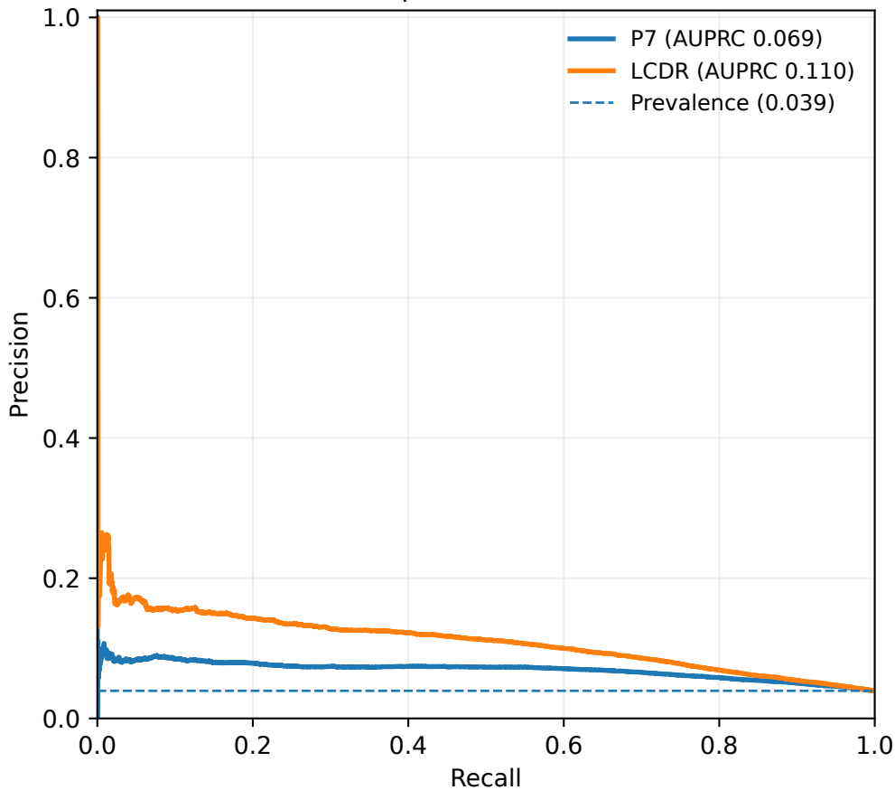
PadChest precision-recall curves
