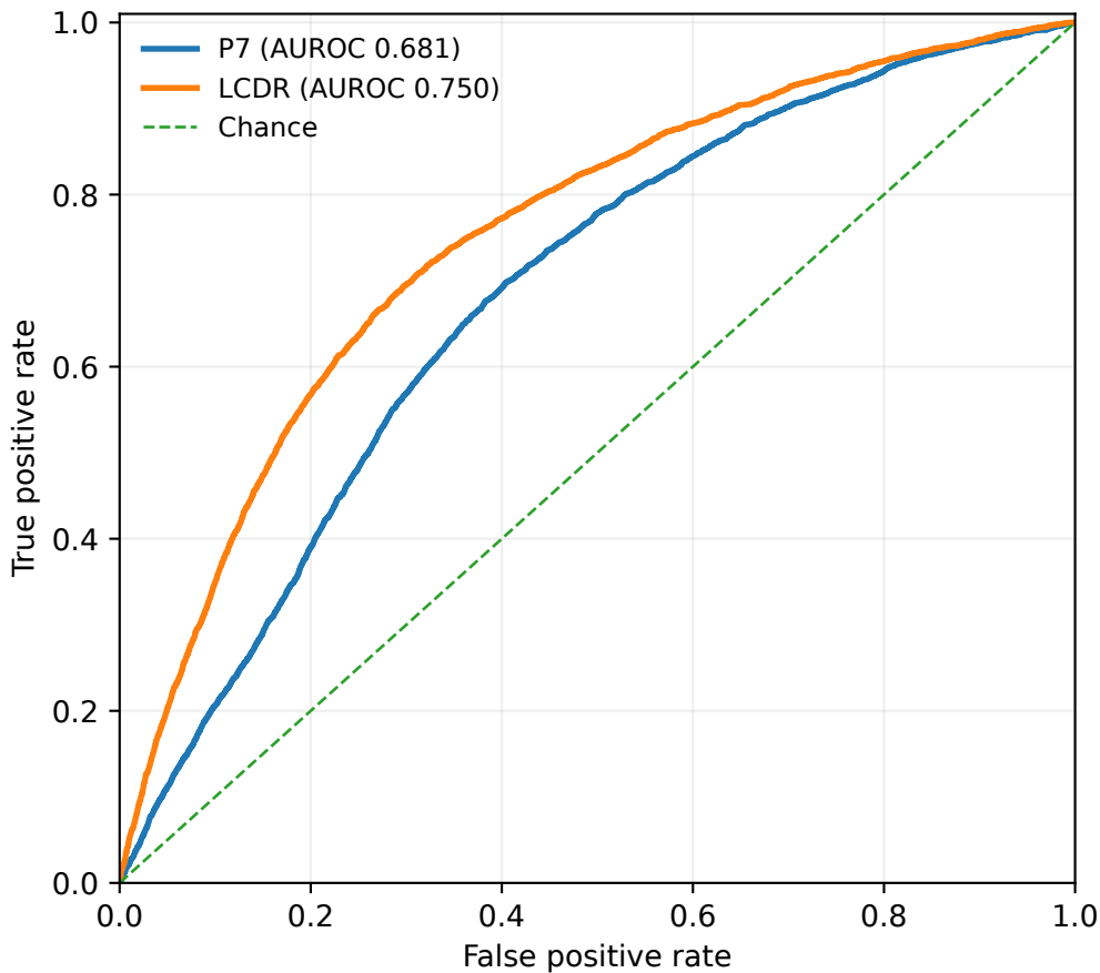
PadChest ROC curves
