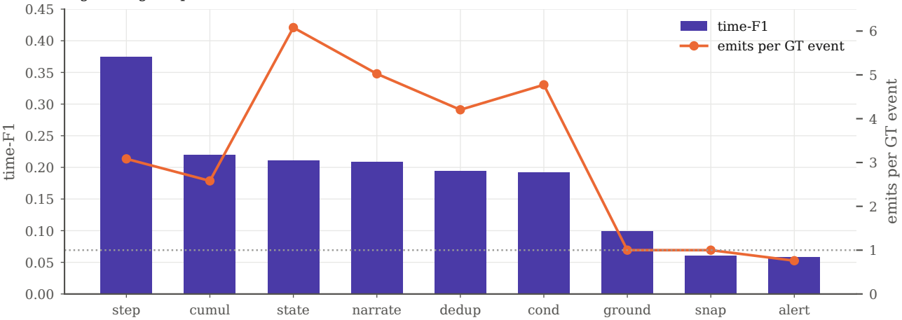
Fig 6 Stage 3, per task: score and the emission ratio behind it
