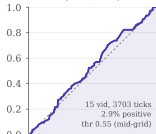
snapshot AUC 0.526 [0.43, 0.63]
