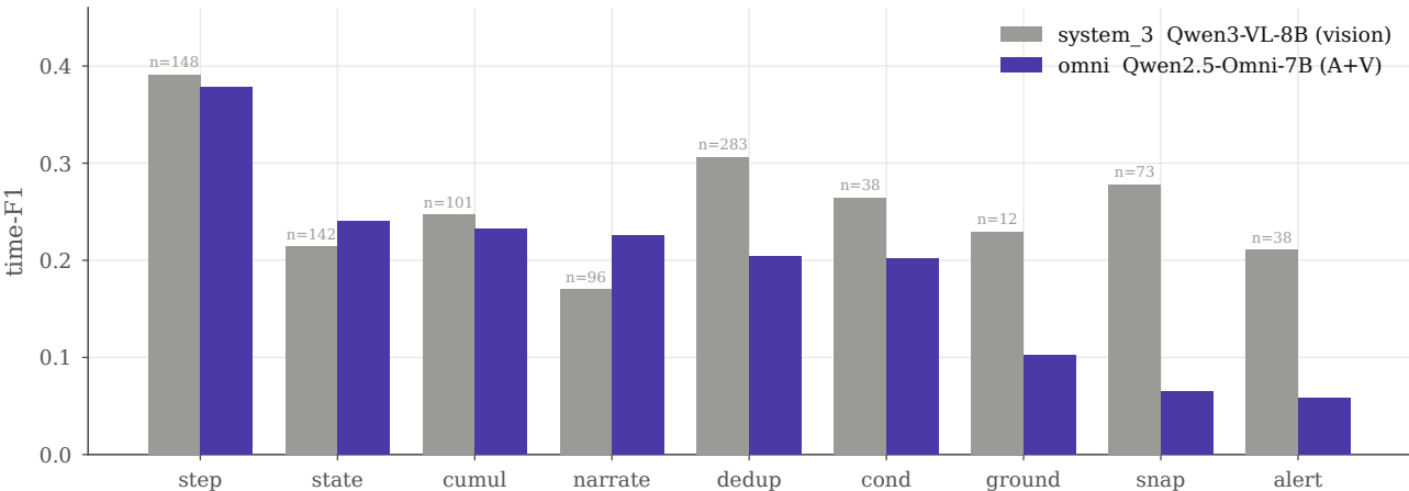
Fig 8 Head to head (time-F1 only; different subsets, see caption)
