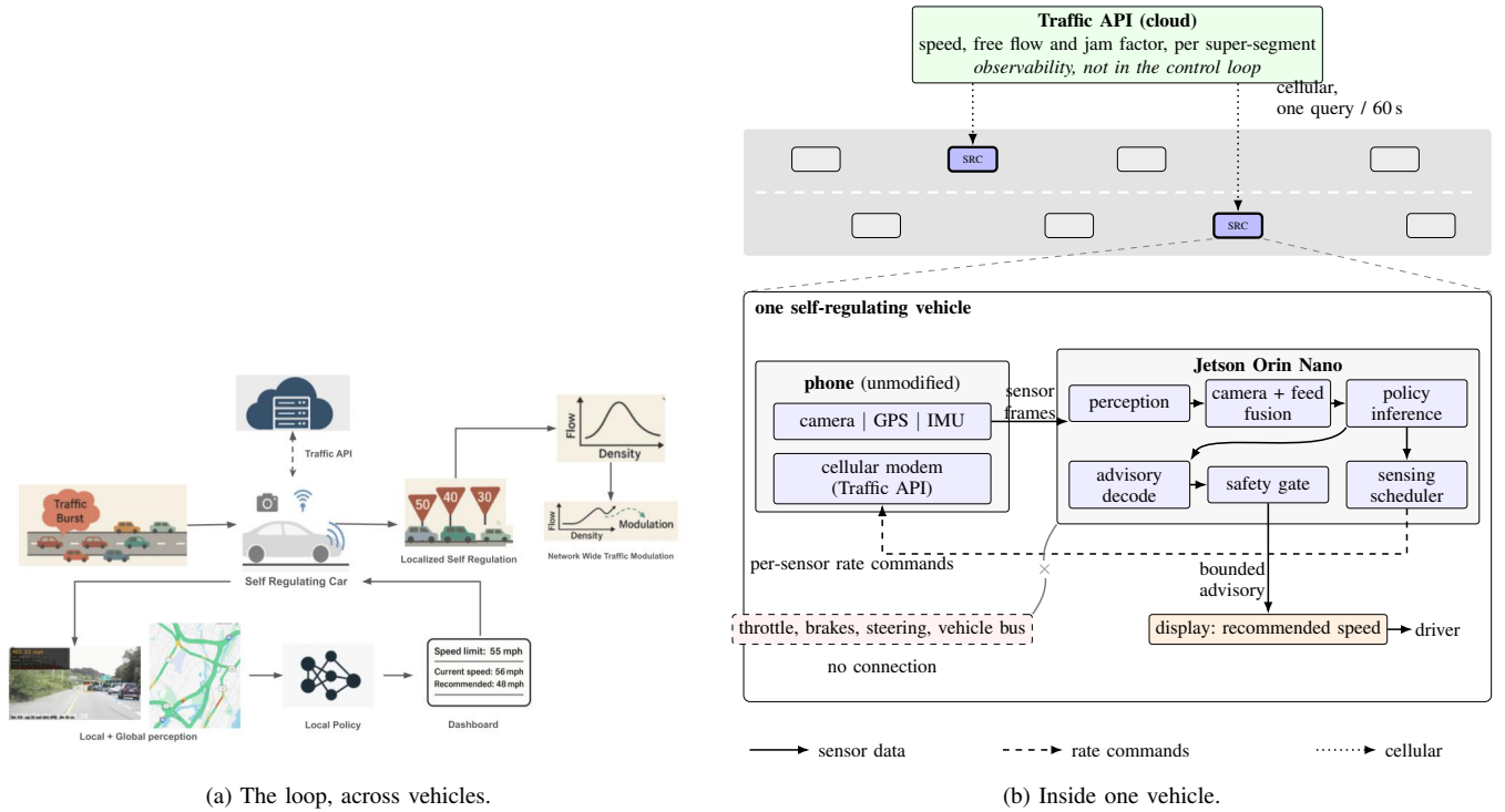
Fig. 2. The deployment, at two scales. In (a) a burst of inflow pushes a stretch of road past its critical density; each self-regulating car reads the network from a traffic API and the road ahead from its own camera, runs the policy locally, and shows the driver a recommended speed. The aggregate of those local actions is what moves the network along its flow-density curve, and no vehicle talks to another vehicle. In (b) one of those vehicles. Ordinary traffic is grey and self-regulating vehicles are blue. The phone captures or queries at the rate it is told and forwards raw data, and every interpretation and sampling decision is on the Jetson. The dashed box is the set of vehicle systems nothing in this design touches.
