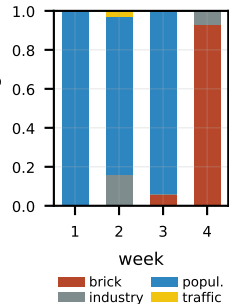
(e) Obs. apportion.
