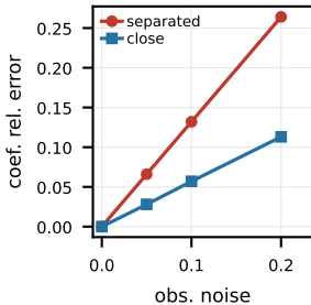
(b) Exp: conditioning
