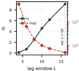
(f) Exp: lag selection
