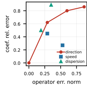
(e) Exp: transport err.
