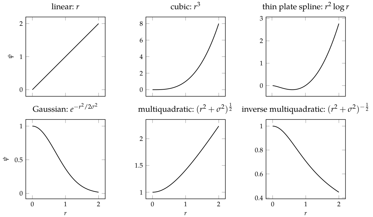
Figure 17.5. Several radial basis functions.
