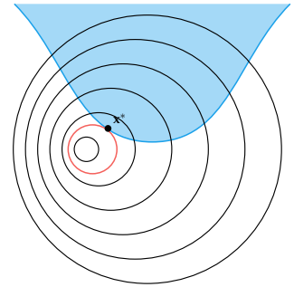
Figure 10.7. An active inequality constraint. The corresponding contour line is shown in red.
