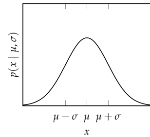
Figure C.6. A univariate Gaussian distribution, \mathcal{N}(\mu, \nu) .
