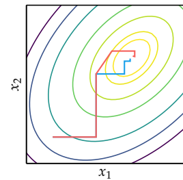
Figure 7.3. Adding the acceleration step to cyclic coordinate descent helps traverse valleys. Six steps are shown for both the original and accelerated versions.
