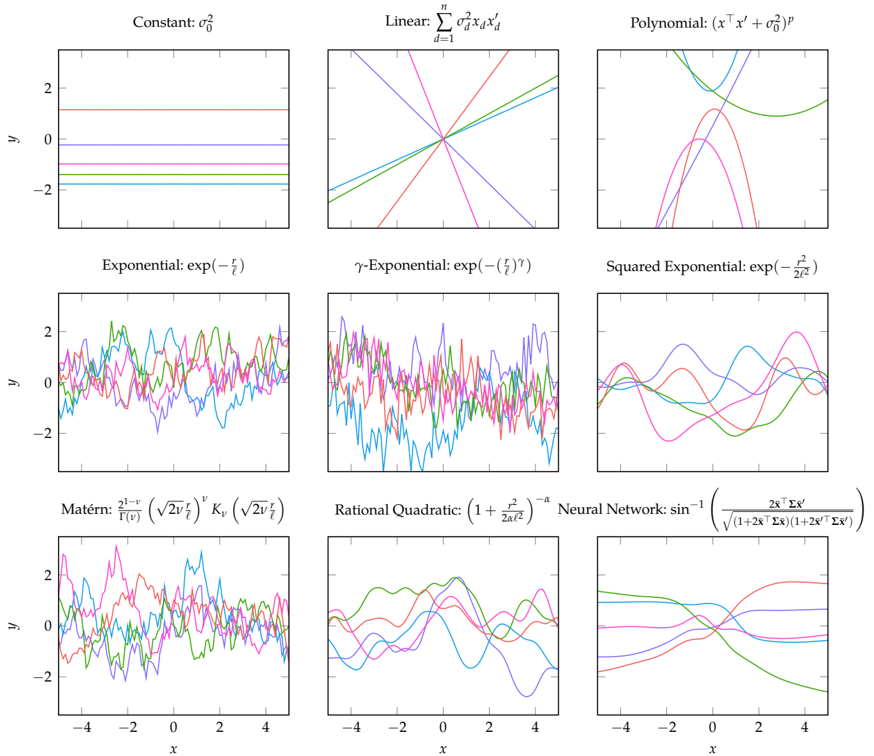
Figure 18.3. Functions sampled from Gaussian processes with different kernel functions. Shown functions are for \sigma_0^2 = \sigma_d^2 = \ell = 1 , p = 2 , \gamma = \nu = \alpha = 0.5 , and \Sigma = \mathbf{I} . In addition, r = \|\mathbf{x} - \mathbf{x}'\| .
