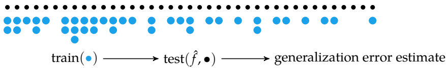
Figure 17.11. A single bootstrap sample consists of m indices into the dataset sampled with replacement. A bootstrap sample is used to train a model, which is evaluated on the full dataset to obtain an estimate of the generalization error.
