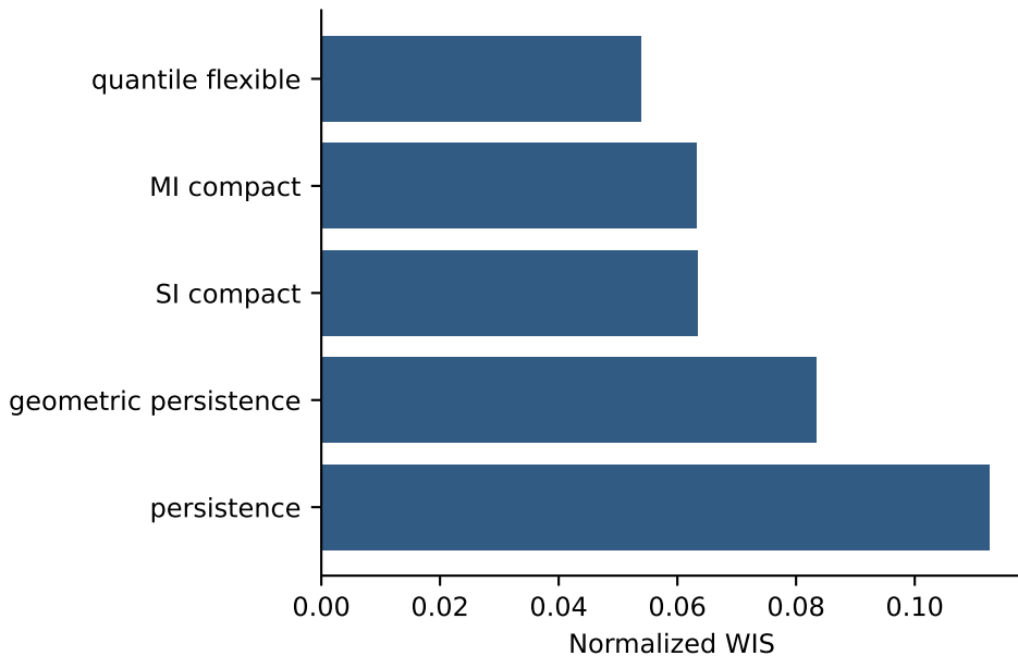
Colorado: score (lower is better)
