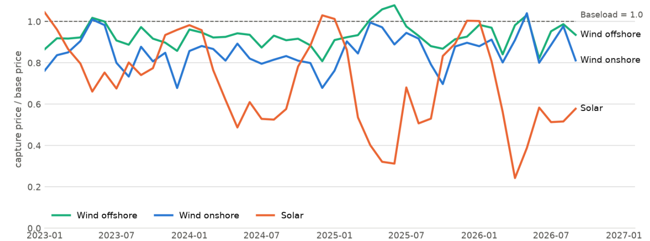
Capture rate by month: what share of the baseload price each technology earns
