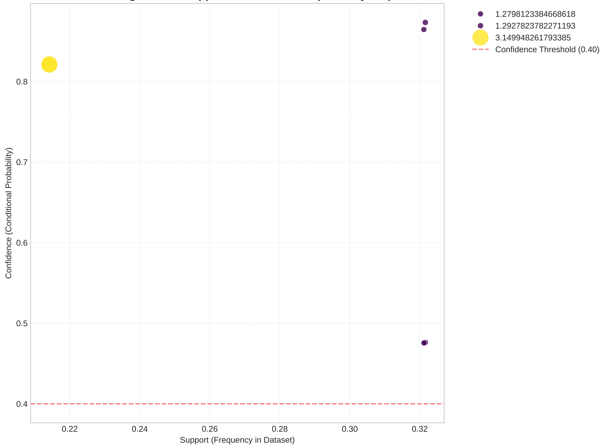
Rule Diagnostics: Support vs. Confidence (Sized by Lift)
